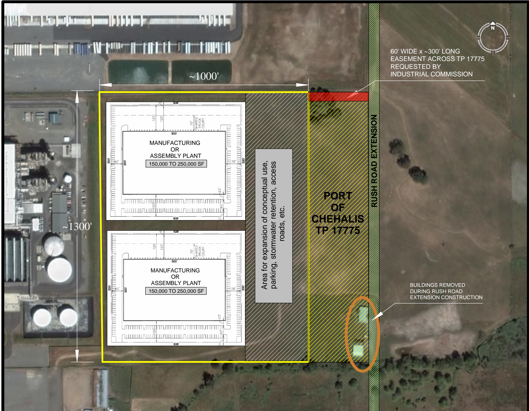
CONCEPTUAL USE OF PARCEL # 17774-1 DRAWING NOT TO SCALE PROPERTY LINES ARE SHOWN FOR REFERENCE ONLY DRAWING ONLY SUGGESTS A DEVELOPMENT STRATEGY
